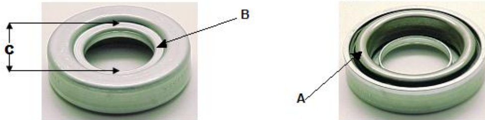
BRG- 2188 – Self Aligning
